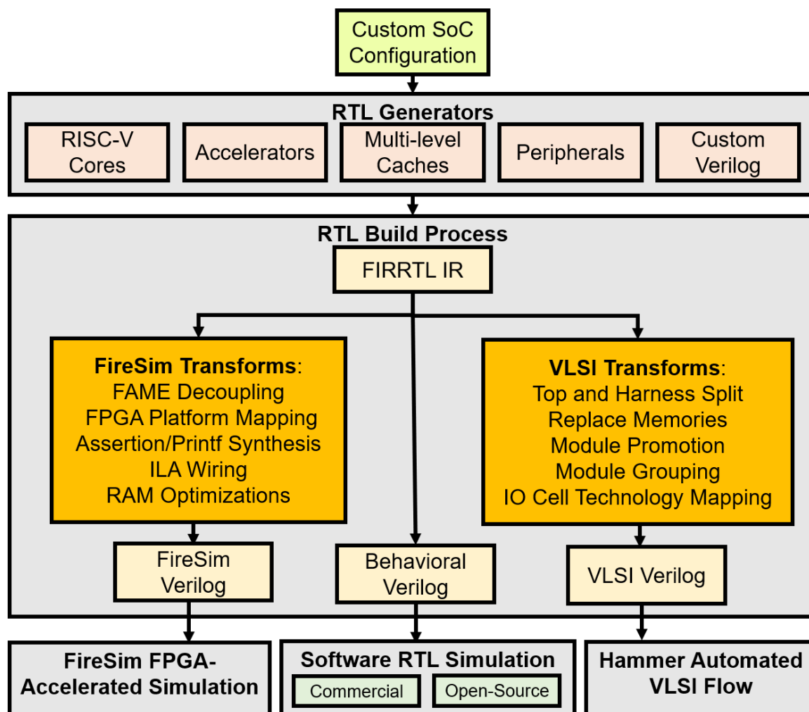
Figure 2. Multiple disparate design flows supported by the Chipyard framework through generators and transformations. A series of FIRRTL transformations consumes generators with a custom configuration, and outputs appropriate Verilog and associated collateral for different design stage platforms.
